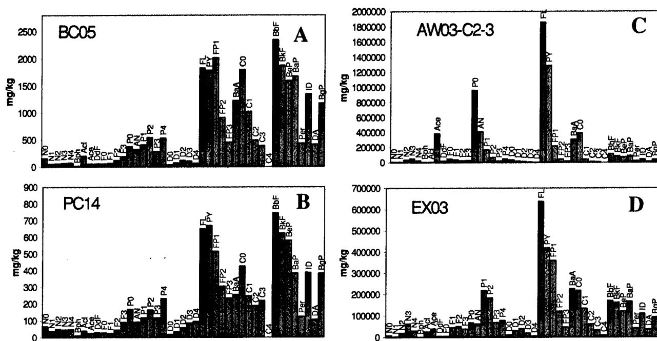
Figure 2-18. Histograms showing the distribution of individual PAH in selected sediments identified as 'end-members' in PC-1 (Figure 2-18). (A-B) PAH patterns consistent with urban background; (C-D) PAH patterns consistent with variously weathered creosote or creosote blends. Compound abbreviations are listed in Table 2-2.
