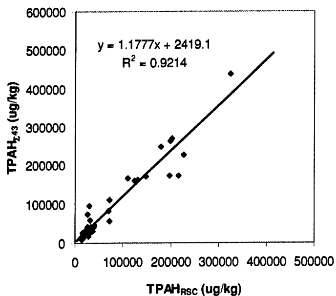
Figure 2-5. Correlation between total PAH determined by RSC ( \text{TPAH}_{\text{RSC}} ; corrected to sum of 16 priority pollutant PAH only) and by ACF ( \text{TPAH}_{\Sigma 43} , includes sum of 43 PAH analytes in Table 2-2). Reduced scale here does not include AW and ER surface and core samples from obvious source areas that were above the calibrated RSC range of 500,000 \mu\text{g/kg} .
