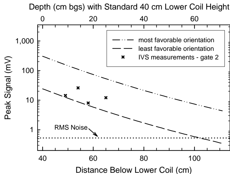
Figure 3-3. EM61-MK2 response curve (time gate 2) for the small ISO
