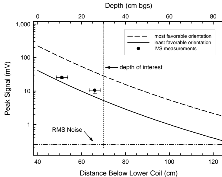
Figure A-7. Calculated response in gate 2 of an EM61-MK2 for a 37-mm projectile in its most and least favorable orientations, the survey noise measured at the site, the signal measured over the two projectiles in the IVS, and an indication of the depth of interest for this item at this site. The error bars correspond to a 2.5-cm (1") uncertainty in the burial depth and 2x the measured amplitude noise.
