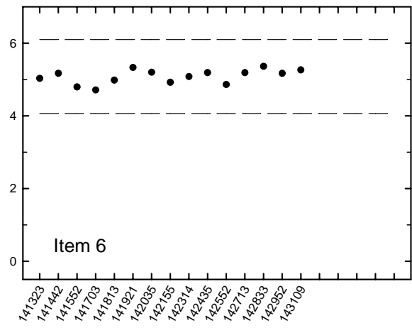
Figure A-13. Twice daily variation of measured signal amplitude for the targets in the IVS. All measured signals (circles) within 20% of the mean as indicated by the dotted lines.
