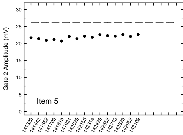
Figure A-13. Twice daily variation of measured signal amplitude for the targets in the IVS. All measured signals (circles) within 20% of the mean as indicated by the dotted lines.
