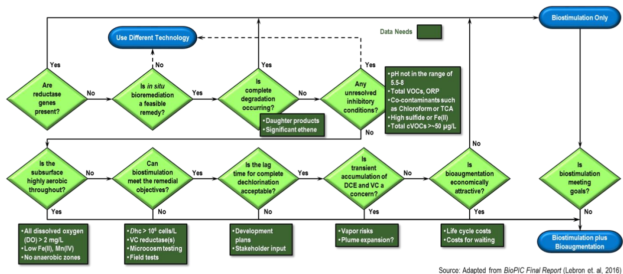
Figure 1. Stepwise Approach to Evaluate Suitability of Reductive Dechlorination and Need for Bioaugmentation (Adapted from Lebrón et al., 2016)
