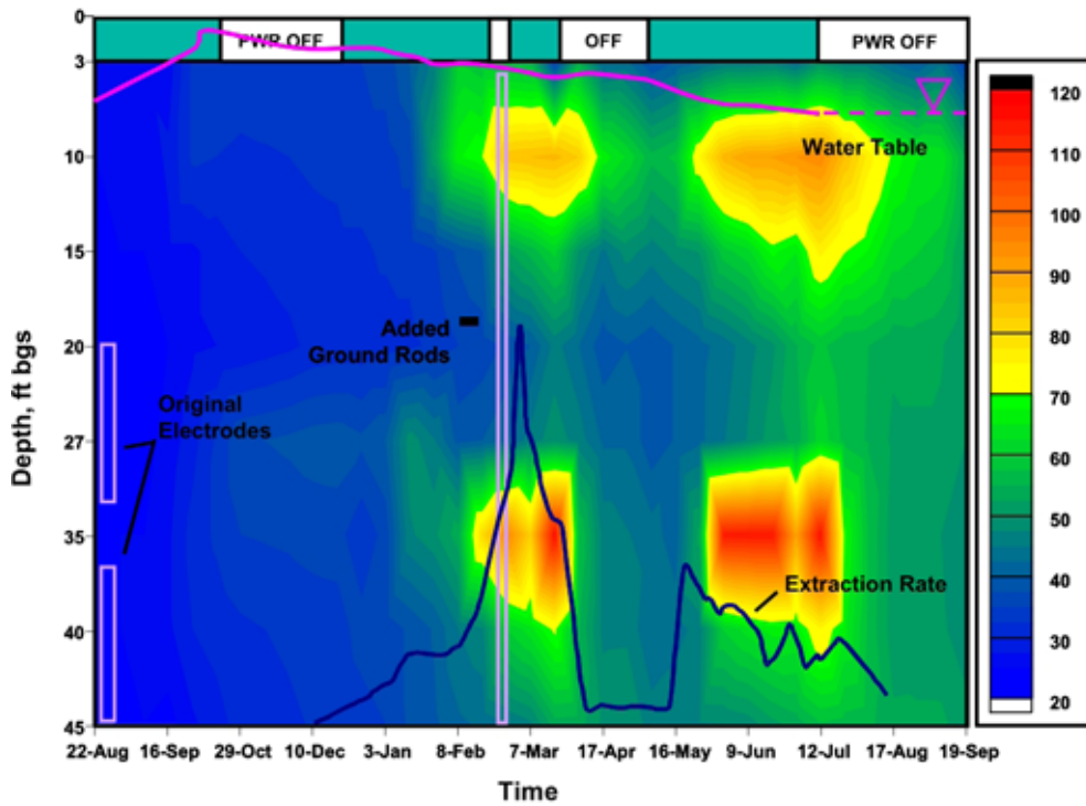
Plot of Subsurface Temperature profiles at TMP 4
