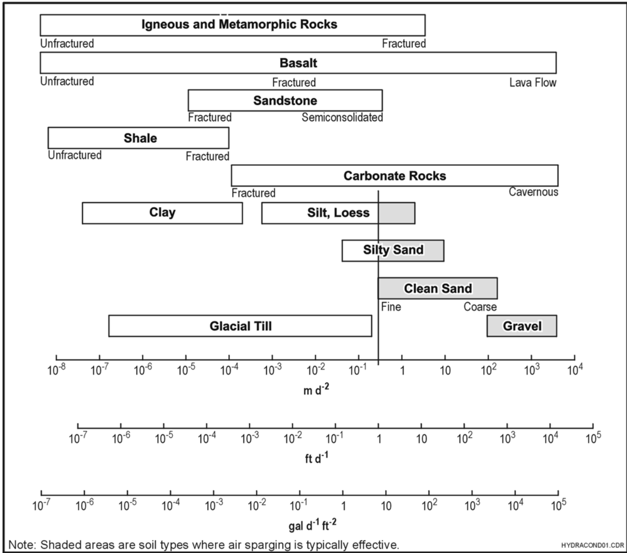
FIGURE D-2. Range of Values for Hydraulic Conductivity and Permeability
