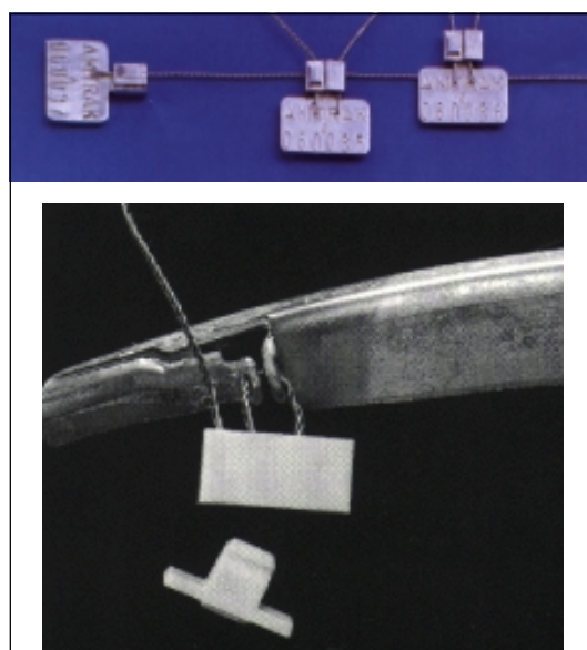
Figure 6-4. Wire and metal crimp seals.
