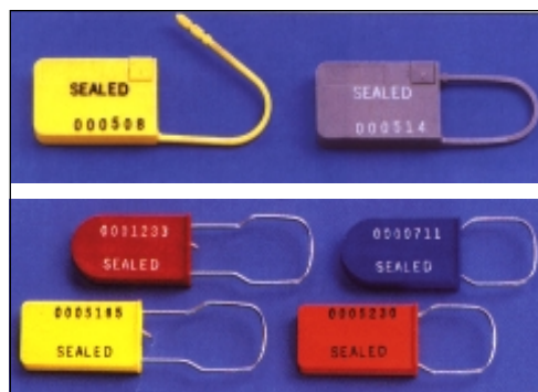
Figure 6-3. Steel and plastic shackle padlock seals.
