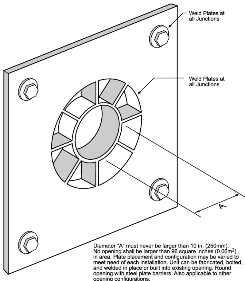
Figure 5-6 Vent and Duct Hardening Barriers
