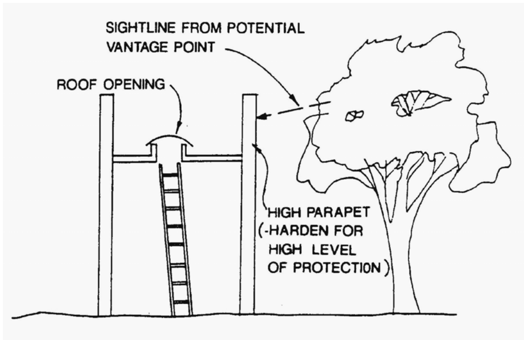
Figure 5-10. Raised Parapets
