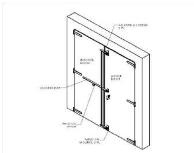
Figure 1. Magazine Door Closure System.
