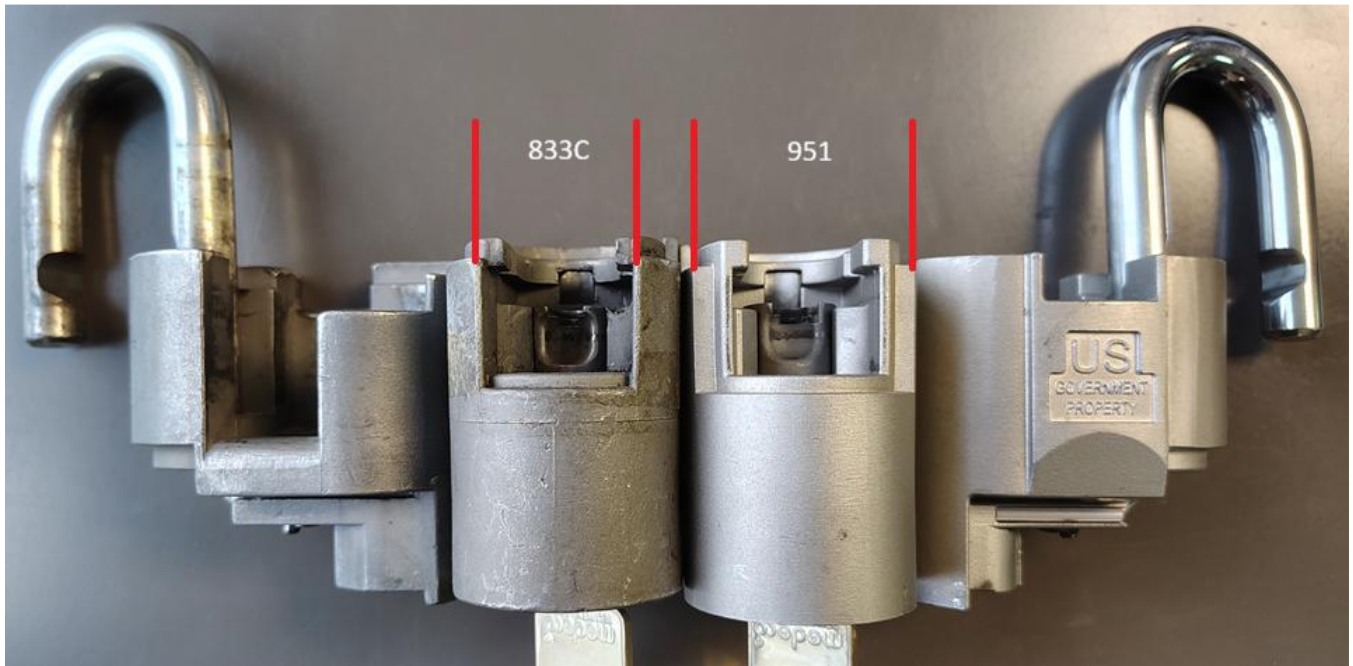
833C and 951 partially disassembled
